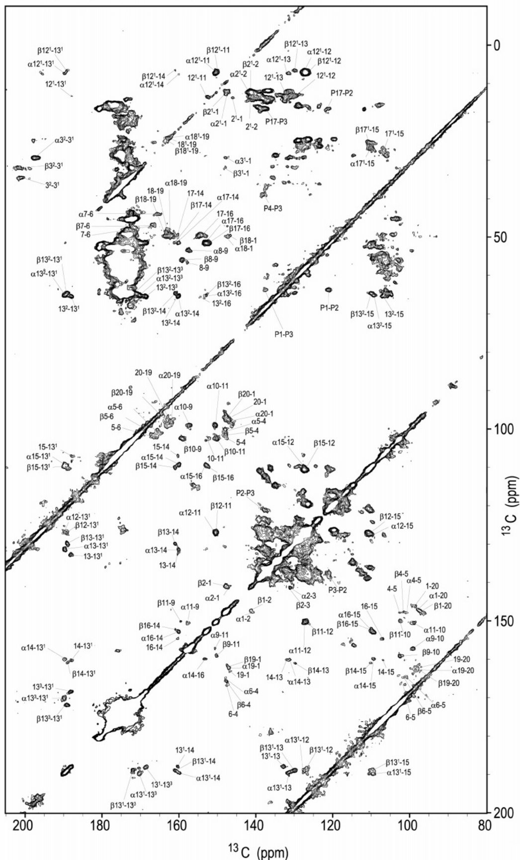
Figure 1. Contour plot of a high-resolution MAS 2D ^{13}\text{C} – ^{13}\text{C} RFDR solid-state NMR spectrum of the [U-^{13}\text{C},^{15}\text{N}] LH2 complex isolated from Rps. acidophila strain 10050. The data were obtained at 223 K with a spinning frequency of 13 kHz and a RFDR mixing time of 2.5 ms. The chemical shift correlation networks of the B800, the \alpha\text{B}850 , and the \beta\text{B}850 are indicated using the IUPAC numbering shown in Figure 2. \alpha\text{B}850 and \beta\text{B}850 are indicated by \alpha and \beta , respectively.
